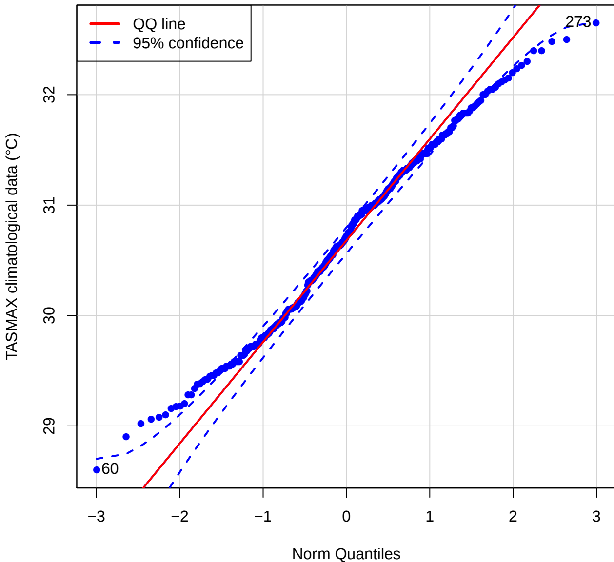
QQ plot (TASMAX of PANS)
