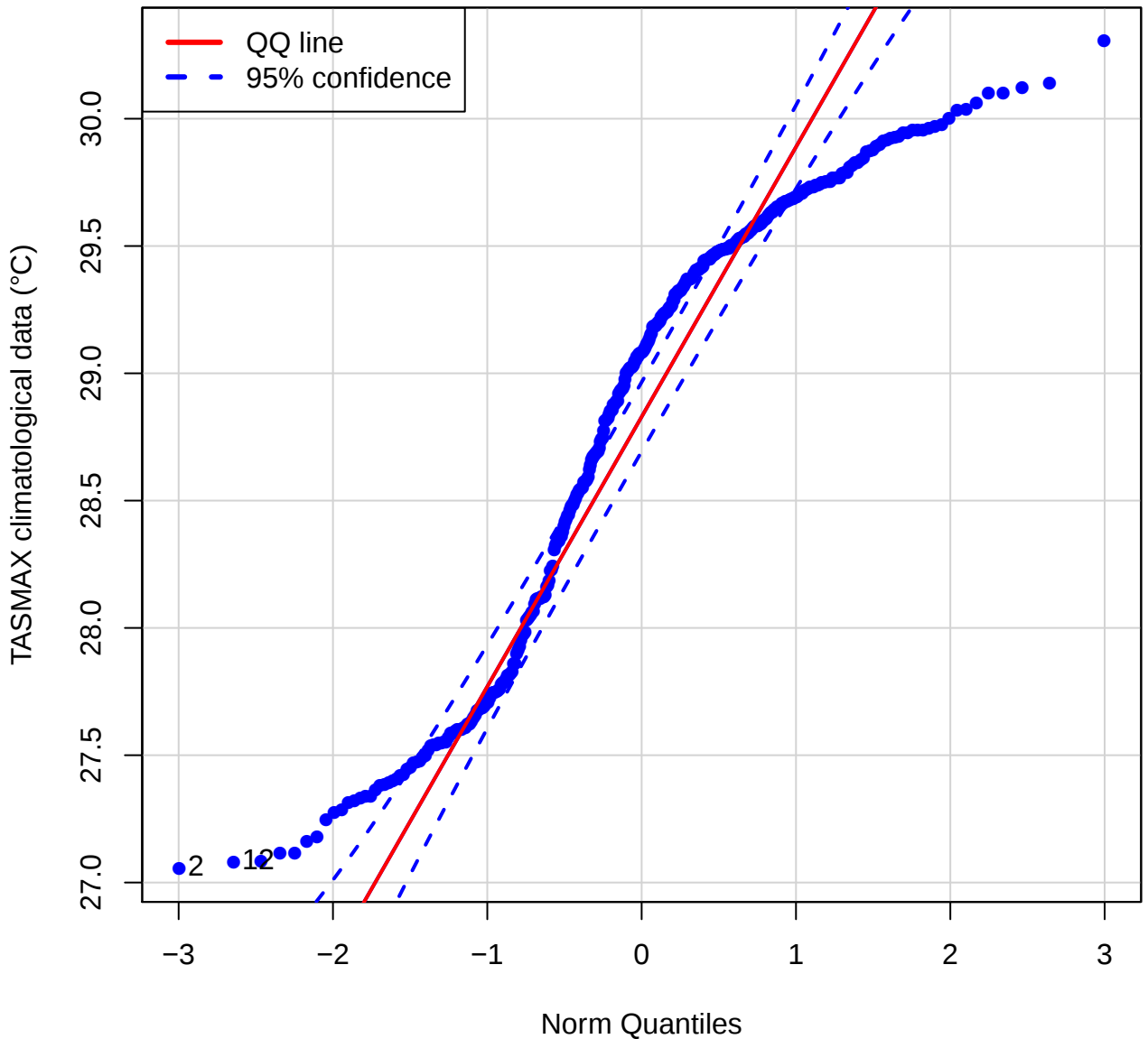
QQ plot (TASMAX of PECH)
