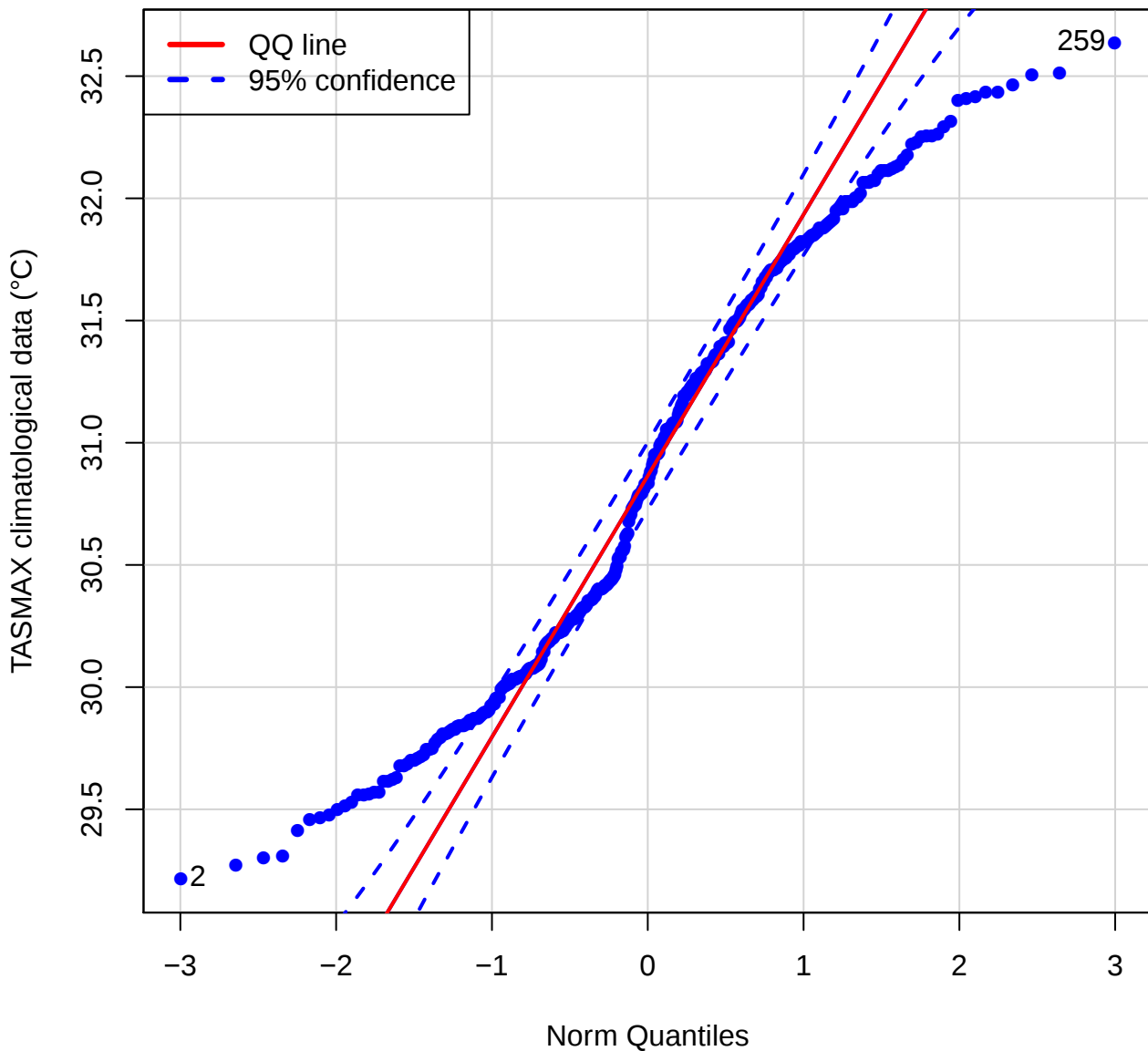
QQ plot (TASMAX of ROBP)
