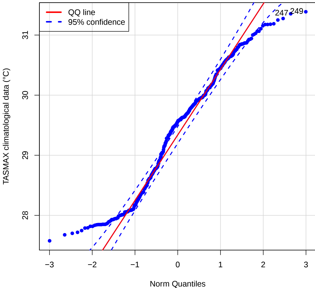
QQ plot (TASMAX of RVPE)
