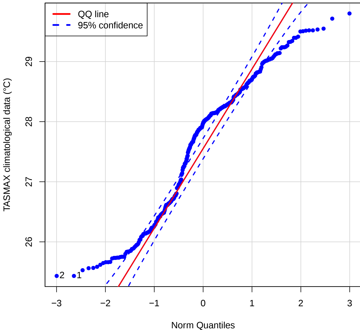
QQ plot (TASMAX of STEB)
