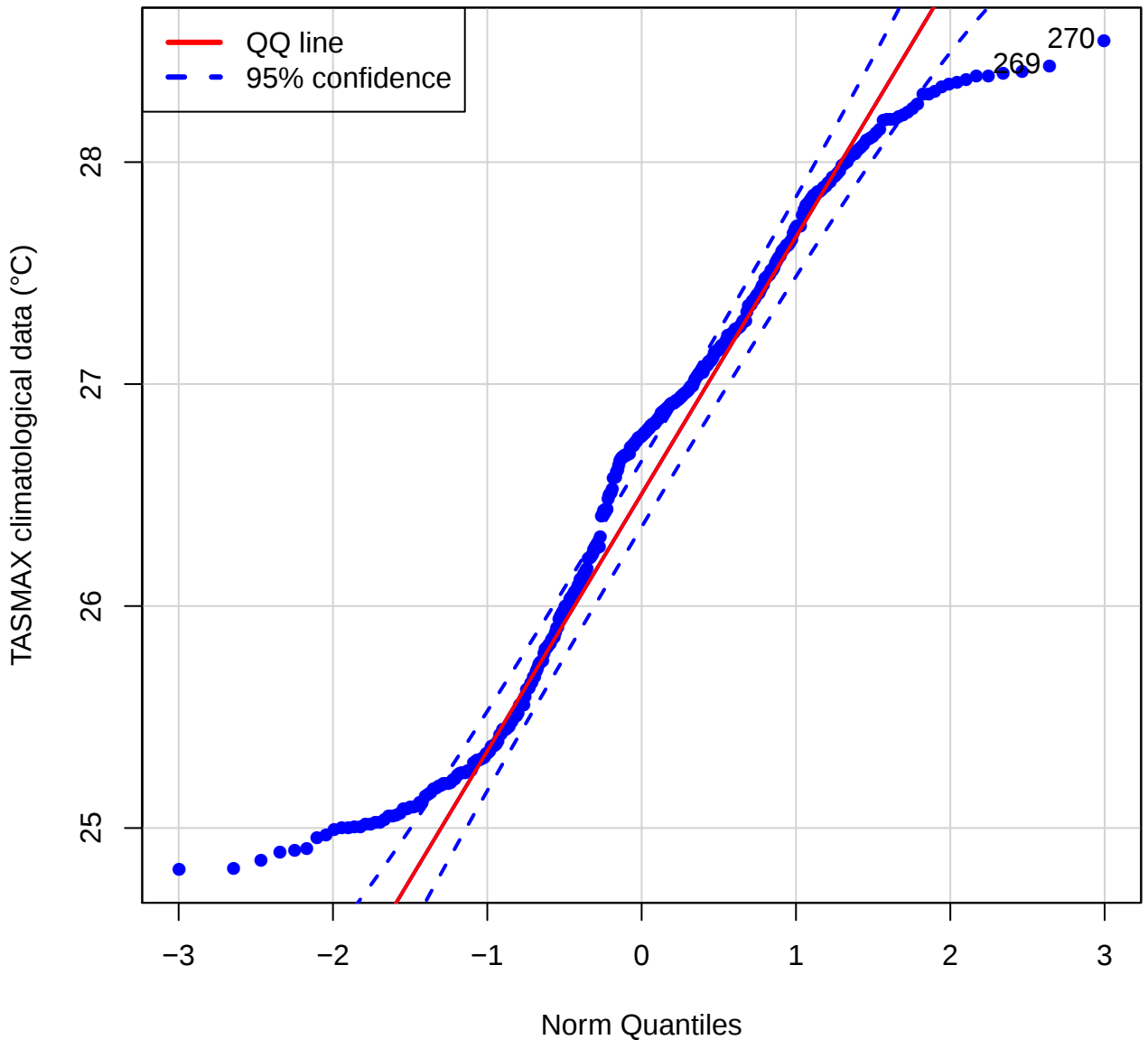
QQ plot (TASMAX of STJB)
