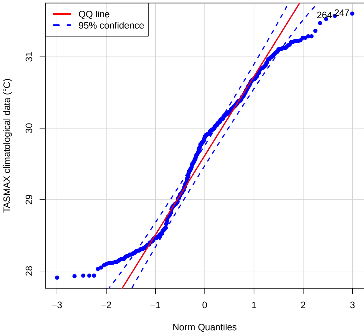
QQ plot (TASMAX of STJL)
