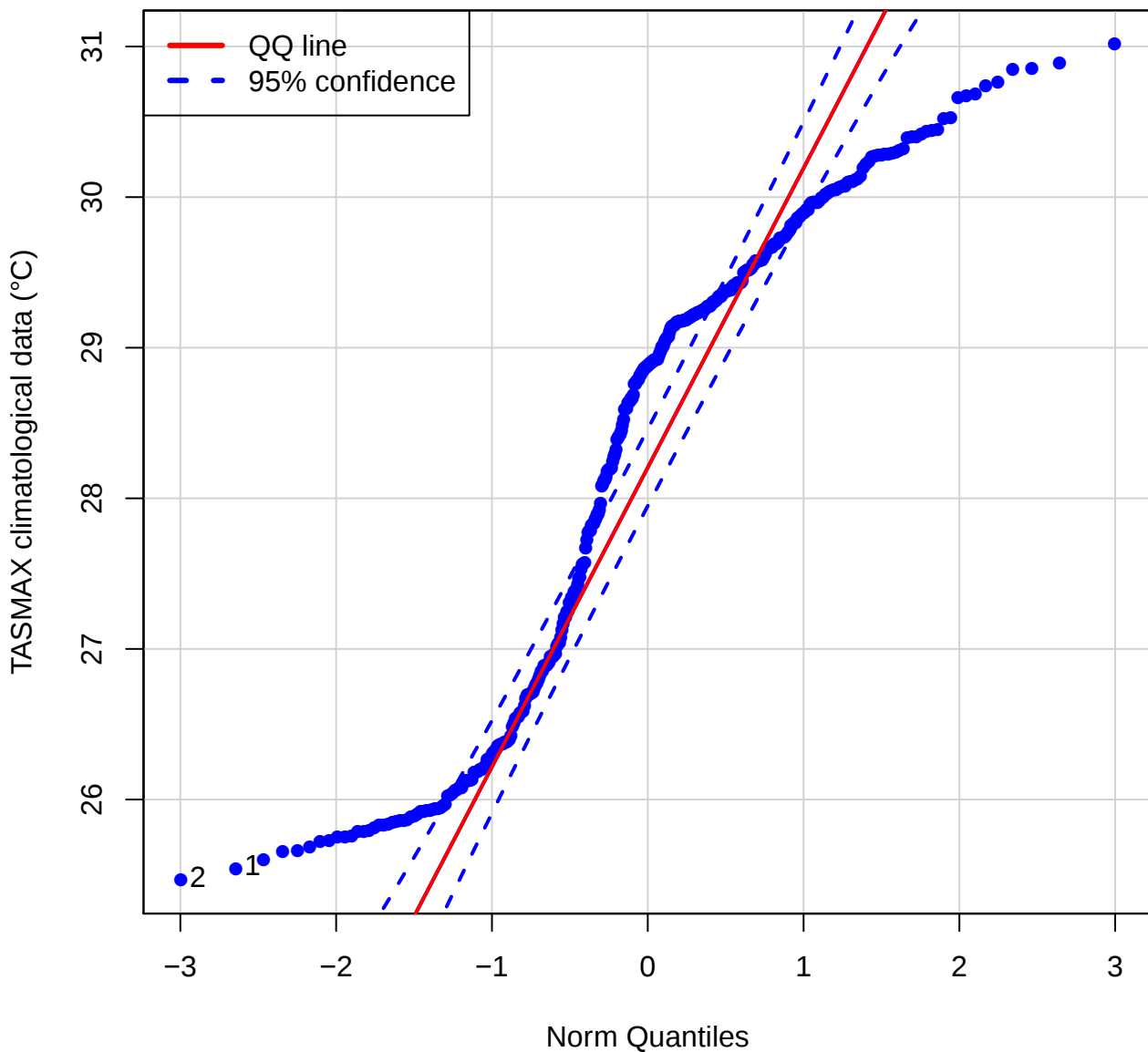
QQ plot (TASMAX of STJO)
