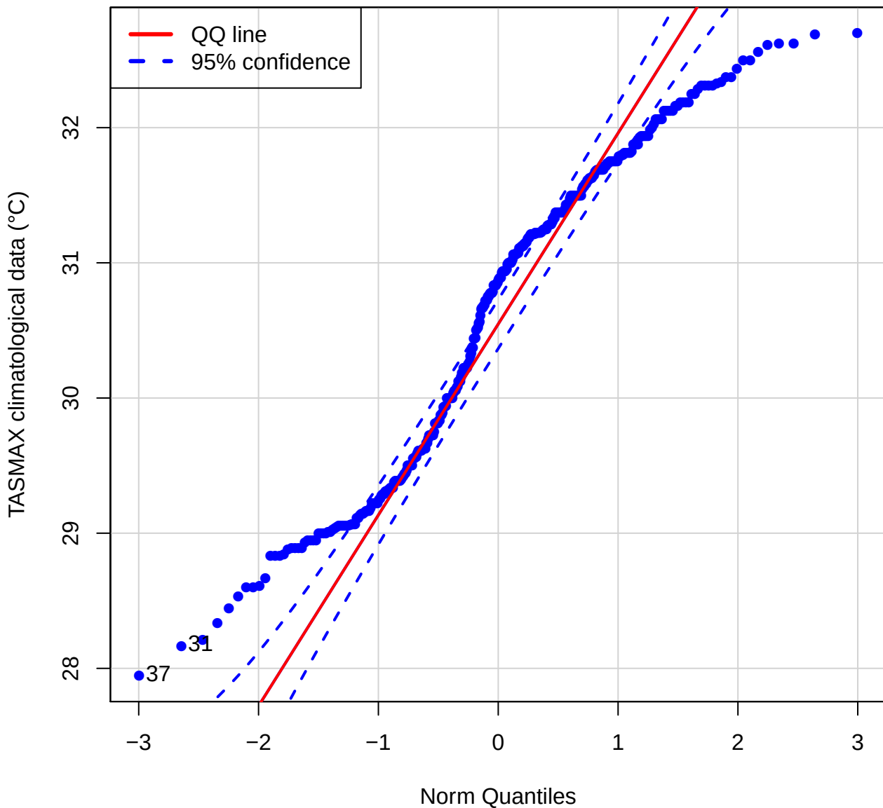
QQ plot (TASMAX of STMB)
