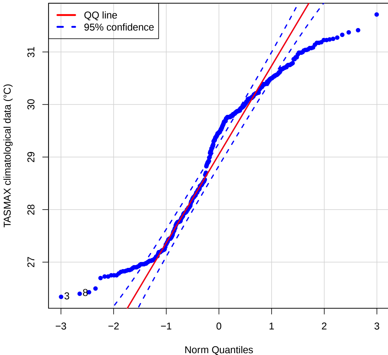
QQ plot (TASMAX of STMC)
