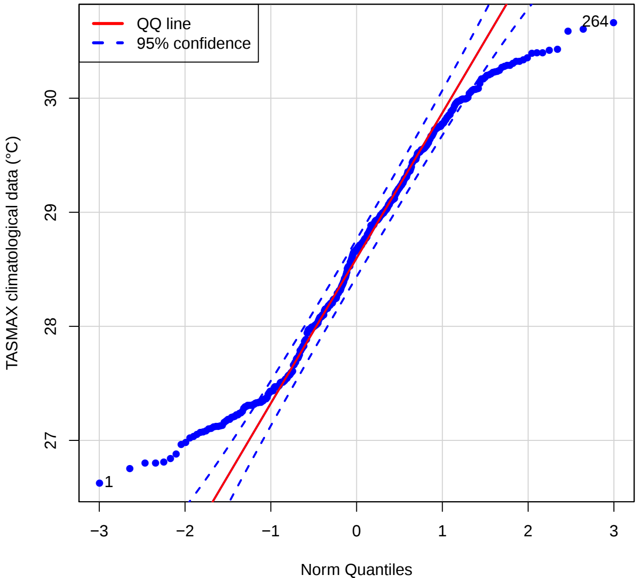
QQ plot (TASMAX of STMP)
