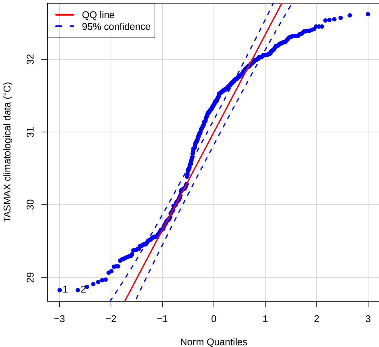
QQ plot (TASMAX of STPR)
