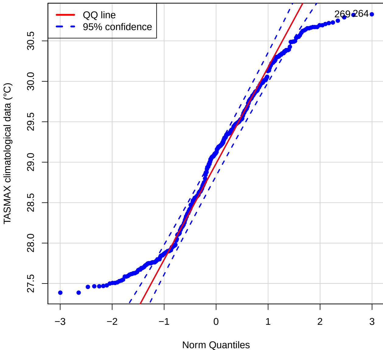
QQ plot (TASMAX of TRTR)
