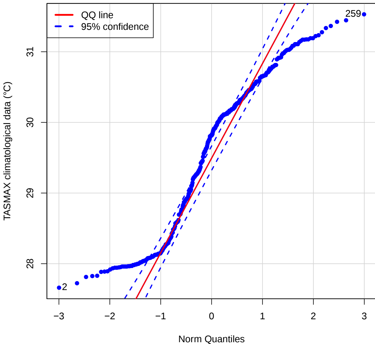
QQ plot (TASMAX of VCLC)
