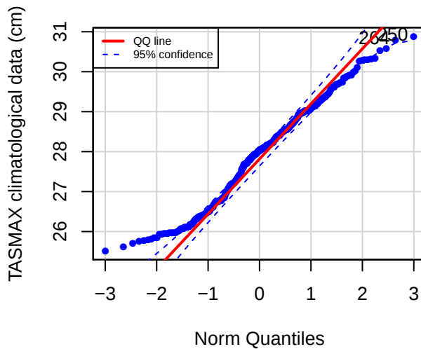
QQ plot (AJPB)
