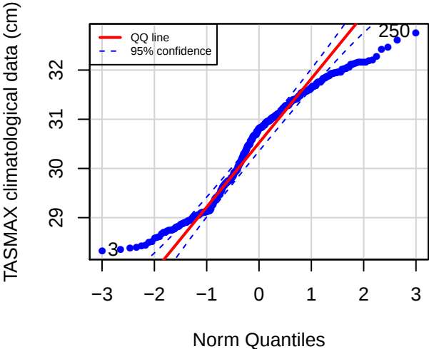
QQ plot (BASP)
