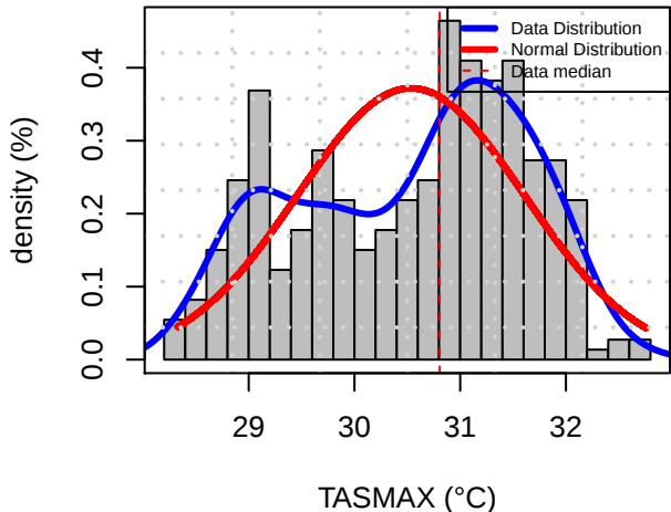
Histogram Distribution (BASP)
