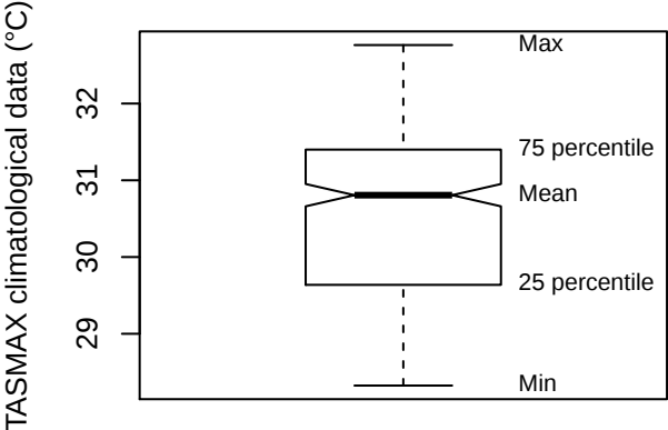
Box plot (BASP)
