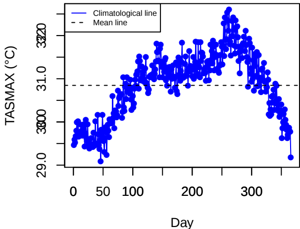
Climatology (DIAM)
