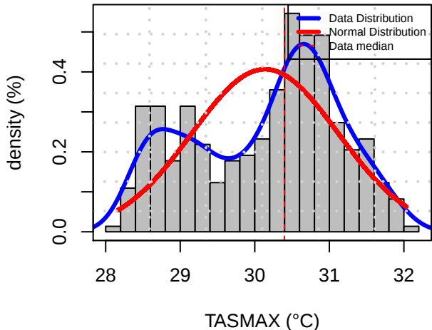
Histogram Distribution (DUCO)
