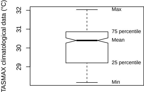
Box plot (DUCO)
