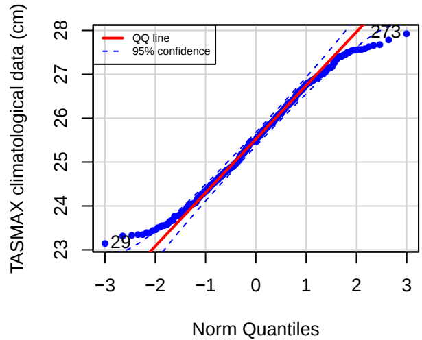
QQ plot (FDFC)
