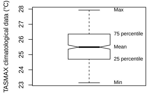
Box plot (FDFC)
