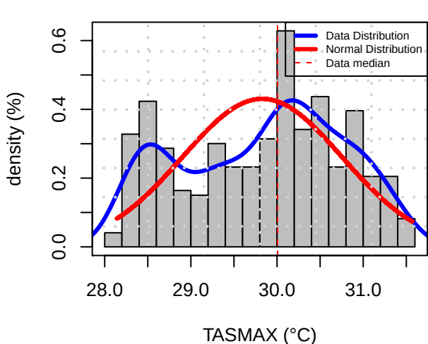
Histogram Distribution (FDFF)
