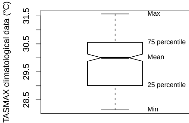
Box plot (FDFF)
