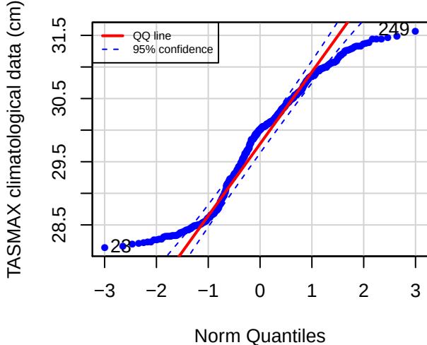
QQ plot (FDFF)
