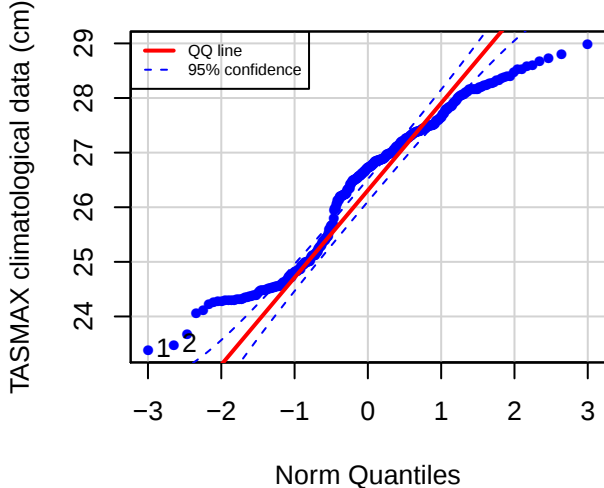
QQ plot (FSDC)
