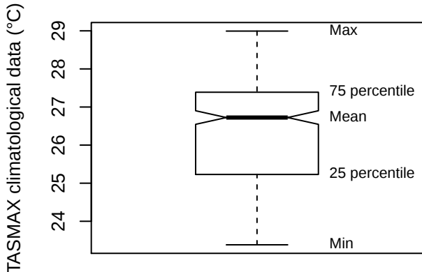
Box plot (FSDC)
