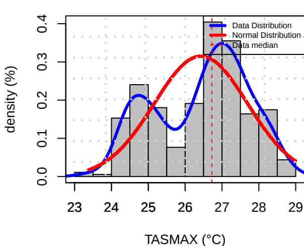
Histogram Distribution (FSDC)
