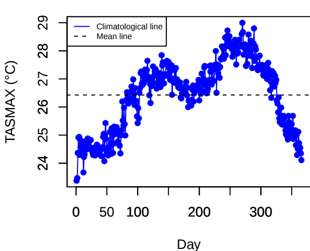
Climatology (FSDC)
