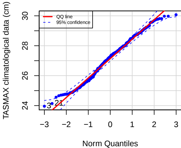
QQ plot (FSDG)
