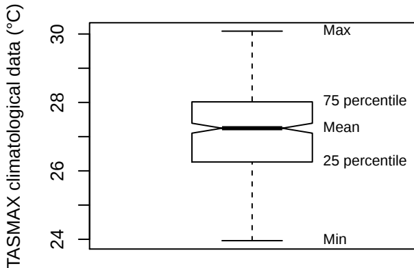
Box plot (FSDG)
