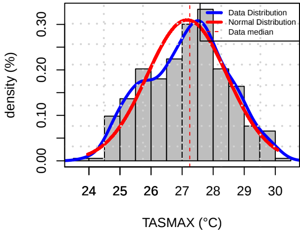
Histogram Distribution (FSDG)
