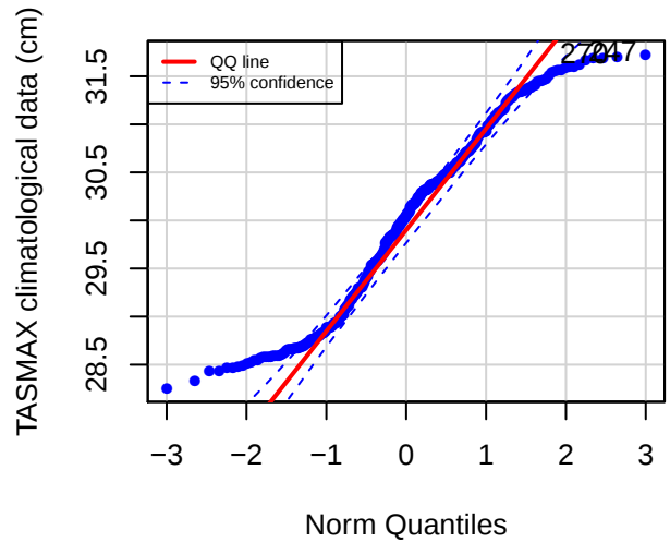
QQ plot (LFRC)
