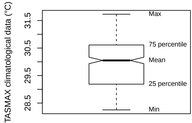
Box plot (LFRC)
