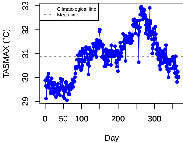
Climatology (LFRS)
