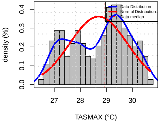
Histogram Distribution (MARB)
