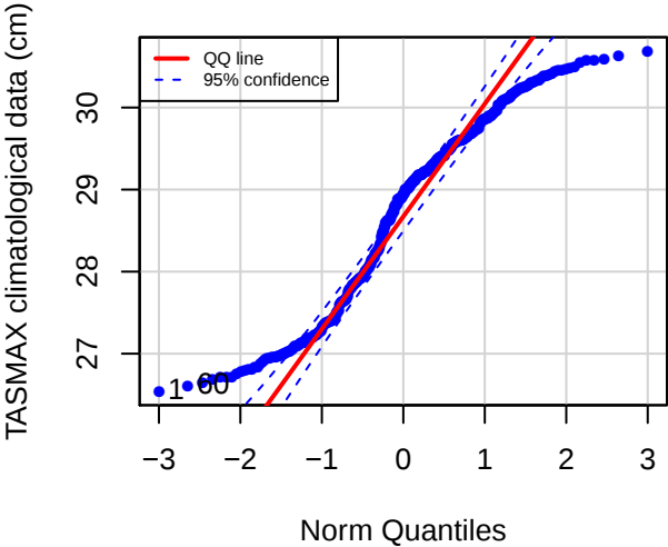
QQ plot (MARB)
