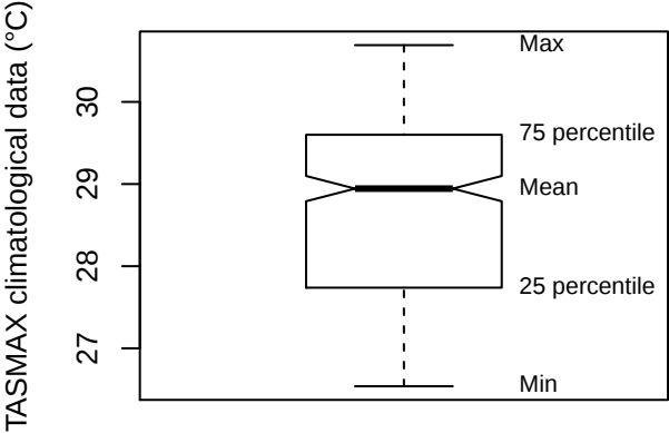
Box plot (MARB)
