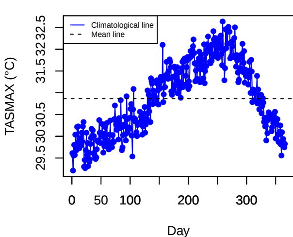
Climatology (ROBP)
