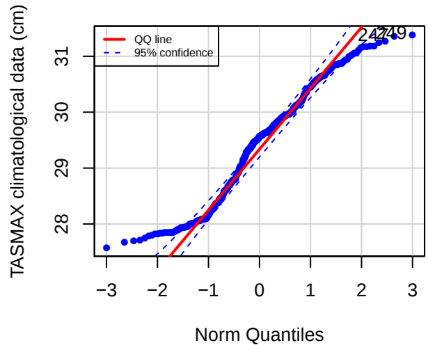
QQ plot (RVPE)
