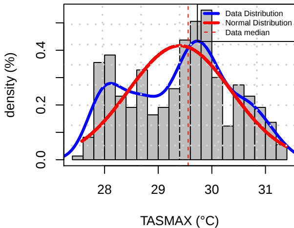
Histogram Distribution (RVPE)
