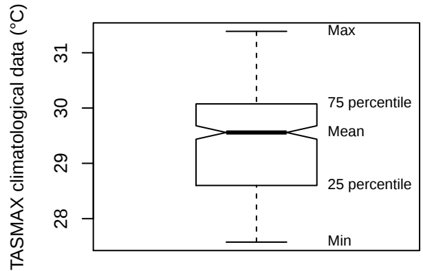
Box plot (RVPE)
