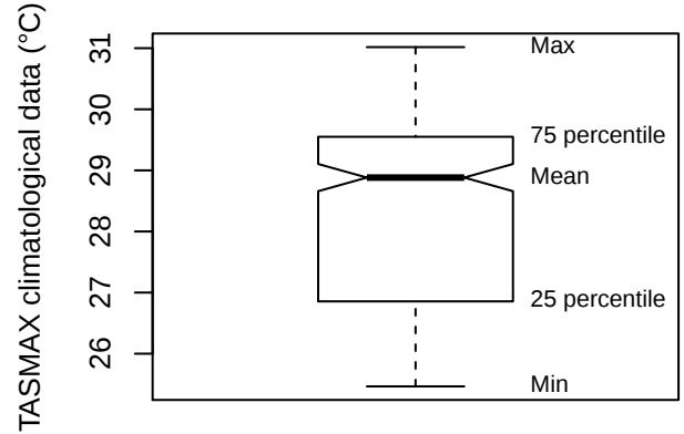
Box plot (STJO)
