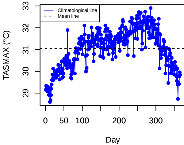
Climatology (STLC)
