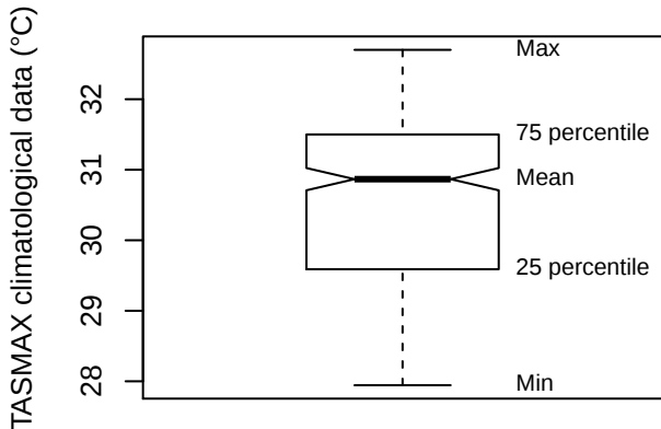
Box plot (STMB)
