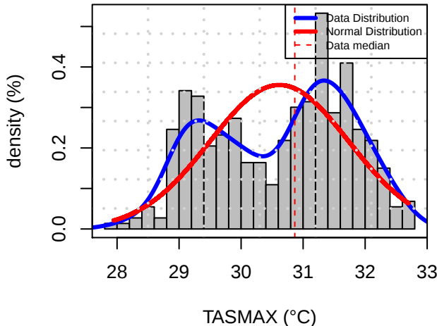
Histogram Distribution (STMB)
