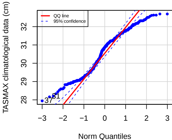
QQ plot (STMB)
