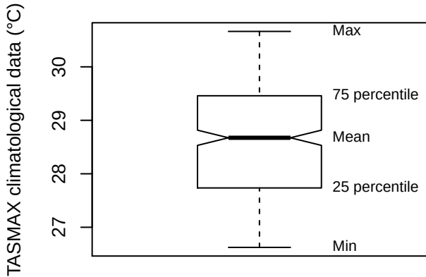
Box plot (STMP)
