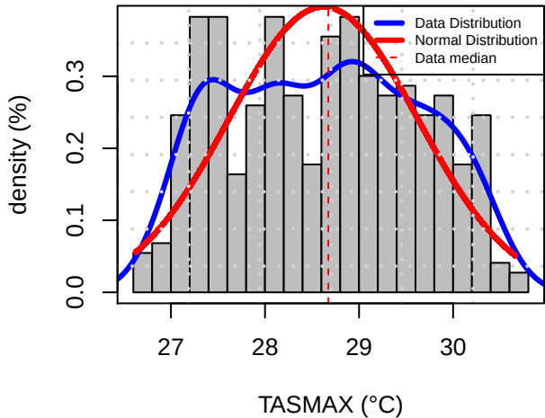
Histogram Distribution (STMP)
