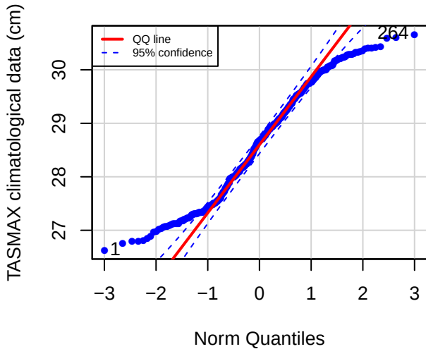
QQ plot (STMP)
