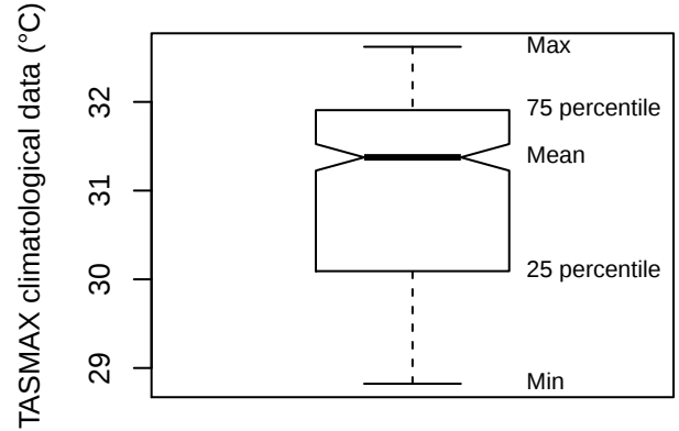
Box plot (STPR)
