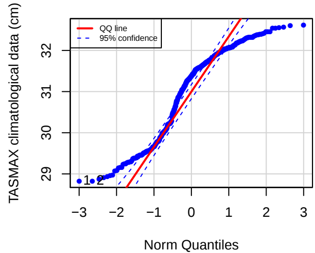
QQ plot (STPR)
