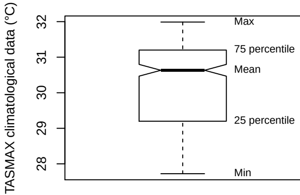
Box plot (TILP)
