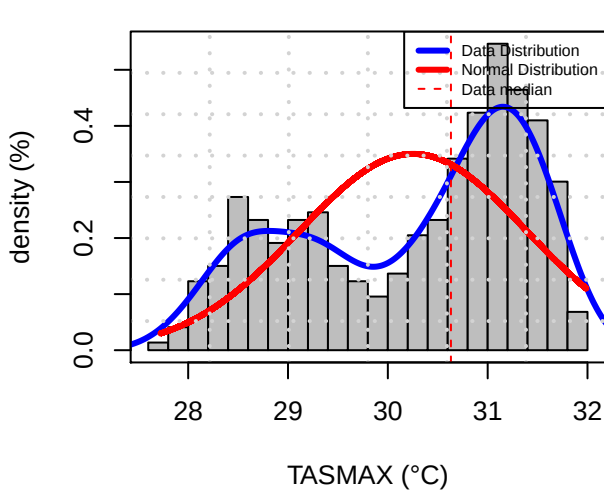
Histogram Distribution (TILP)
