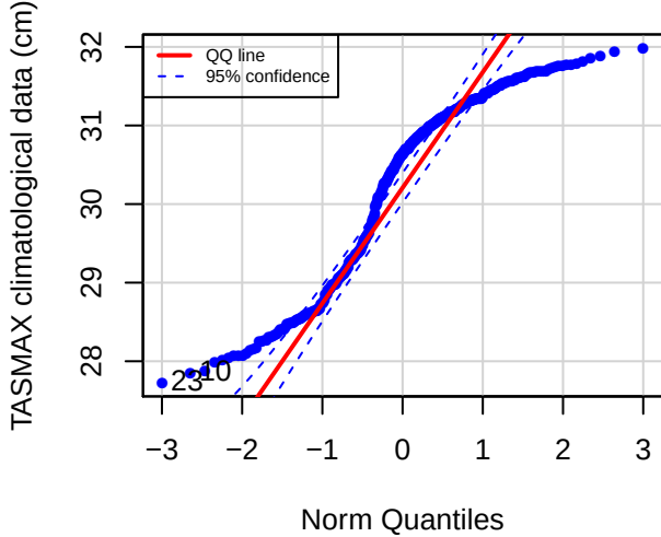
QQ plot (TILP)
