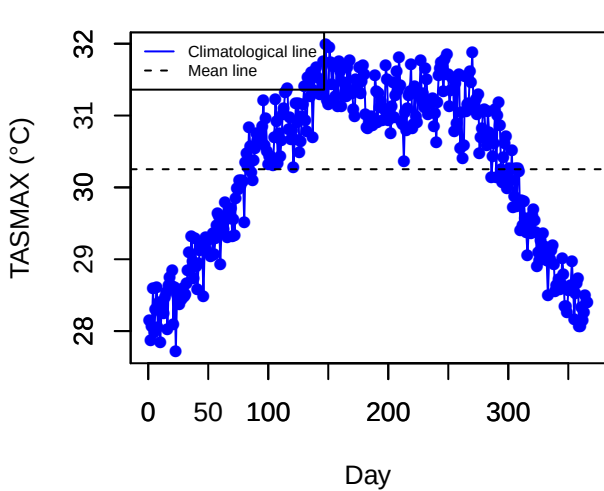
Climatology (TILP)
