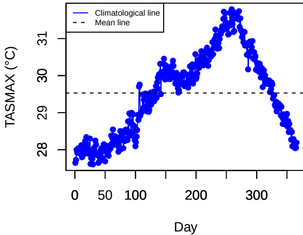
Climatology (TRTC)
