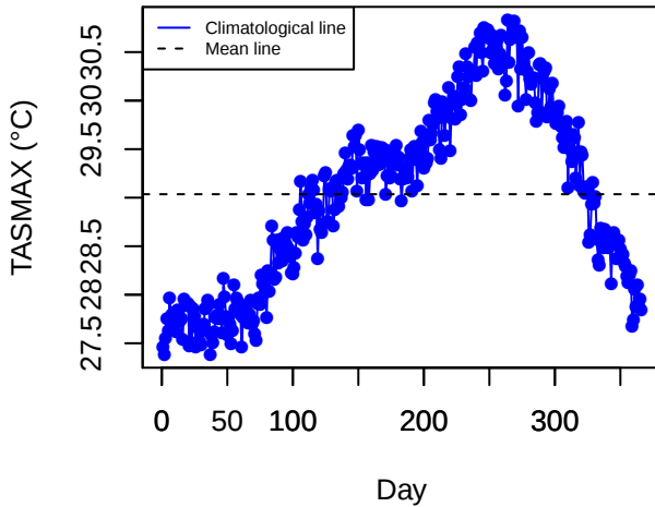
Climatology (TRTR)
