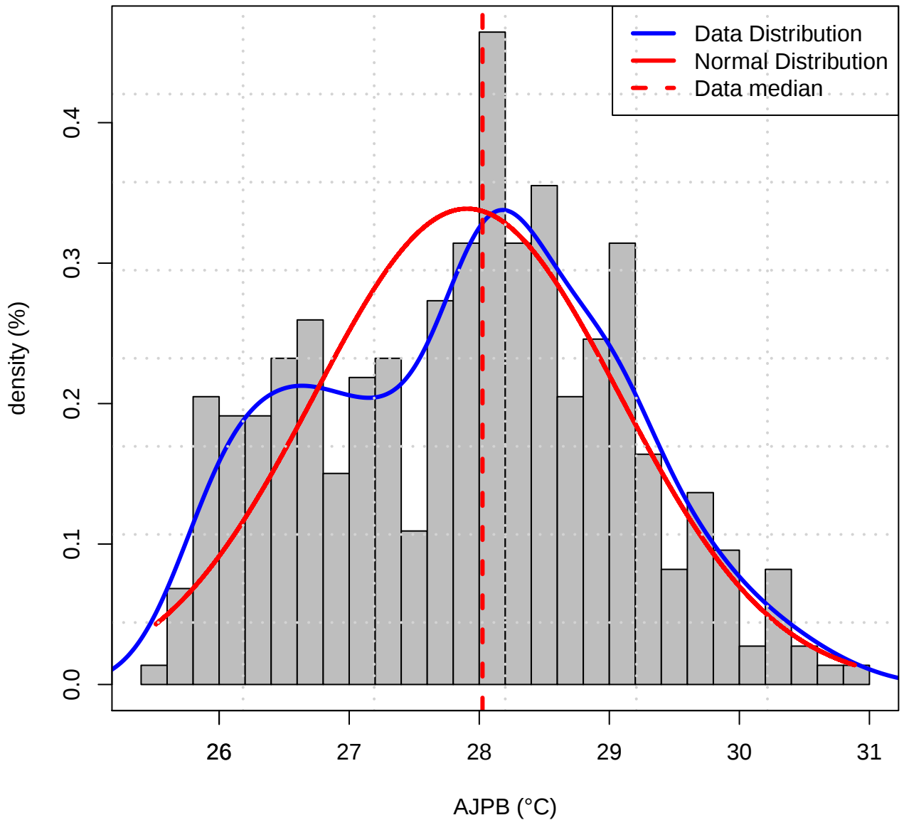
Histogram of Data distribution (TASMAX of AJPB)
