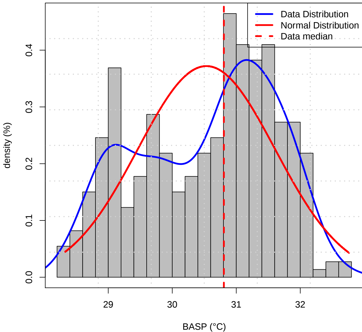
Histogram of Data distribution (TASMAX of BASP)
