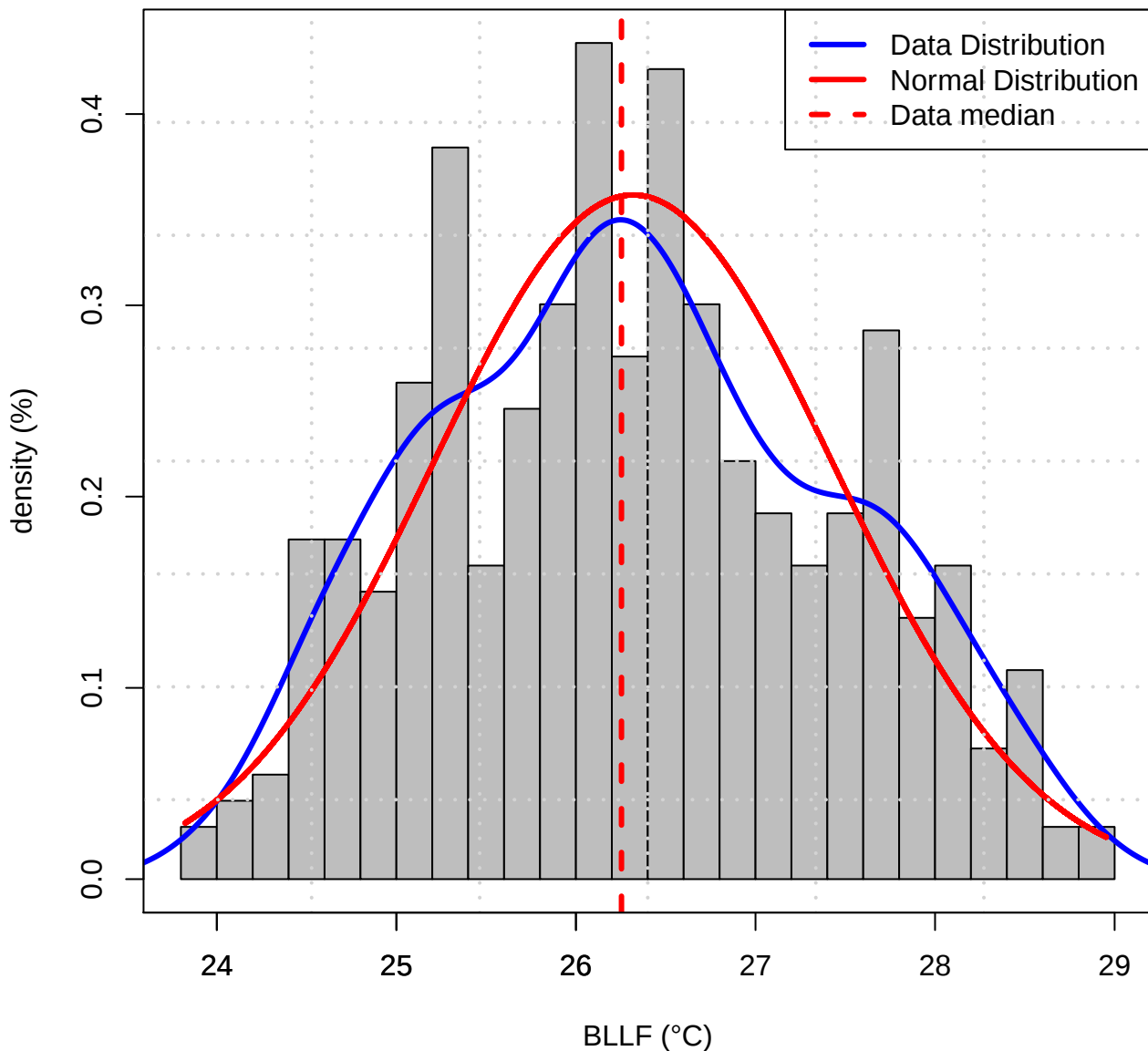
Histogram of Data distribution (TASMAX of BLLF)
