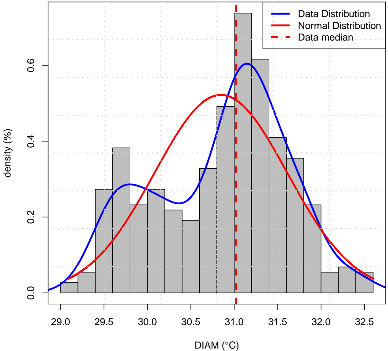
Histogram of Data distribution (TASMAX of DIAM)
