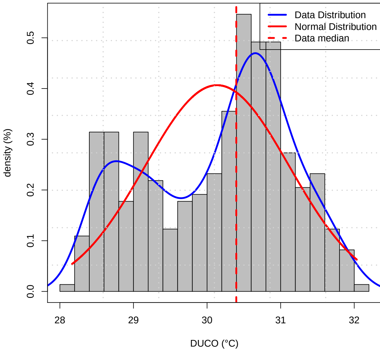
Histogram of Data distribution (TASMAX of DUCO)
