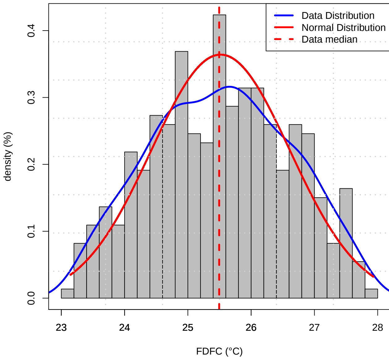
Histogram of Data distribution (TASMAX of FDFC)
