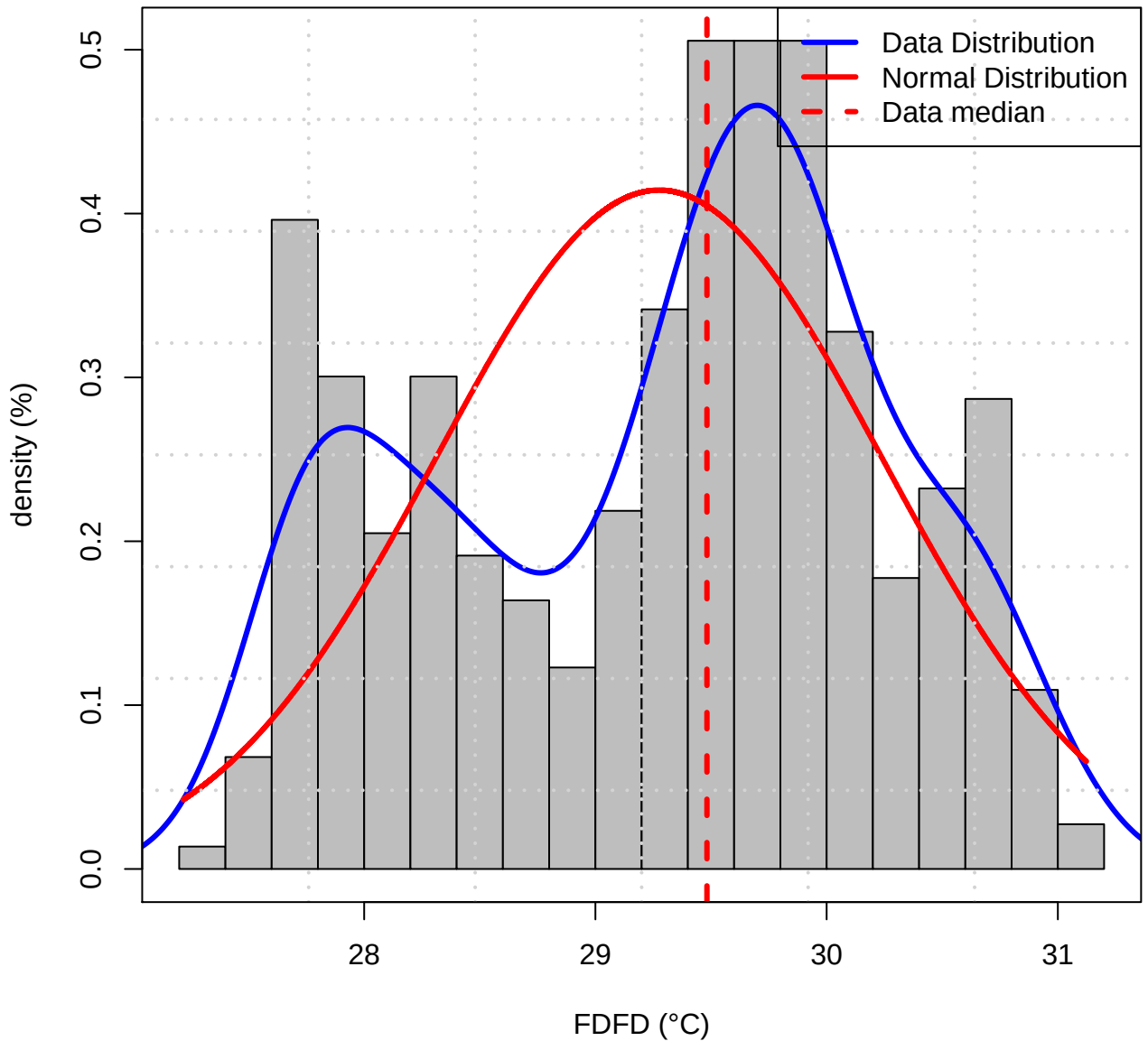
Histogram of Data distribution (TASMAX of FDFD)
