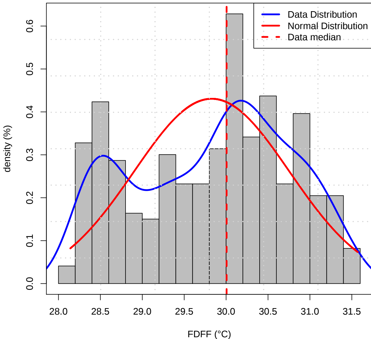
Histogram of Data distribution (TASMAX of FDFF)
