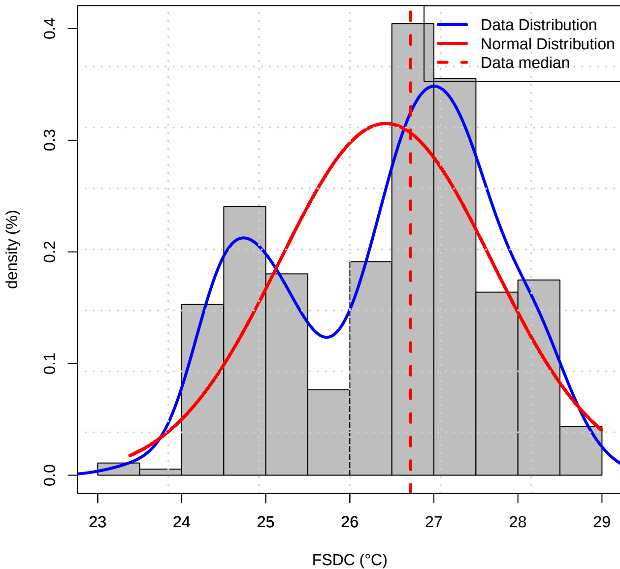
Histogram of Data distribution (TASMAX of FSDC)
