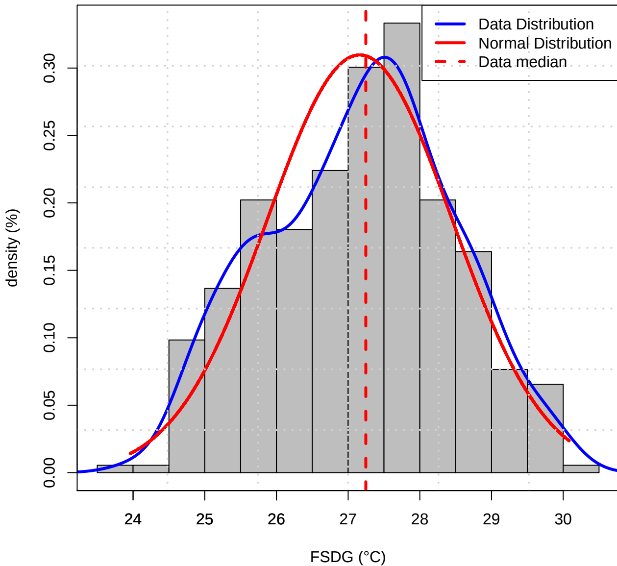
Histogram of Data distribution (TASMAX of FSDG)
