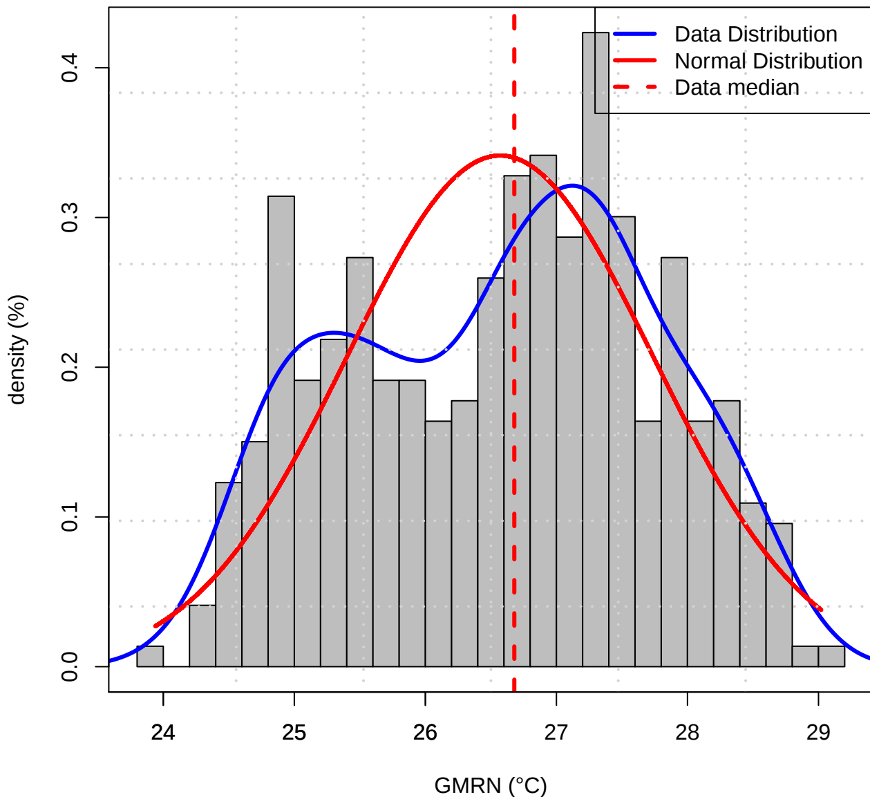
Histogram of Data distribution (TASMAX of GMRN)
