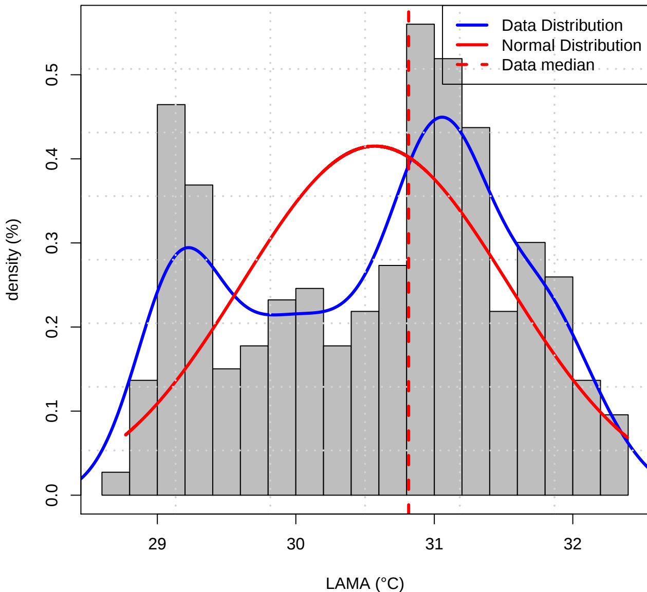
Histogram of Data distribution (TASMAX of LAMA)
