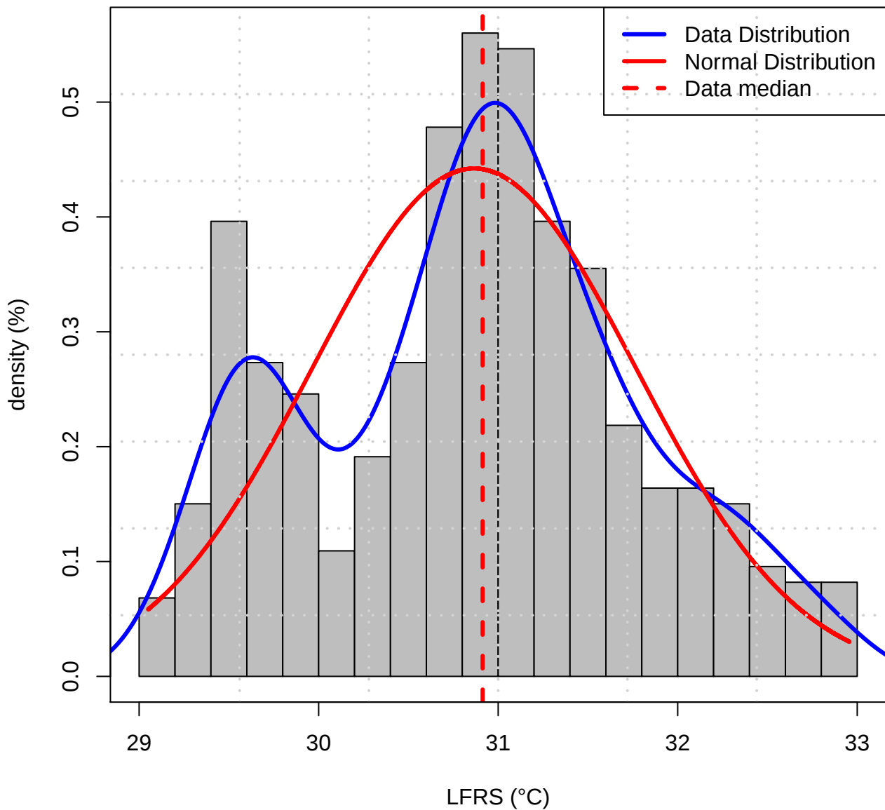
Histogram of Data distribution (TASMAX of LFRS)
