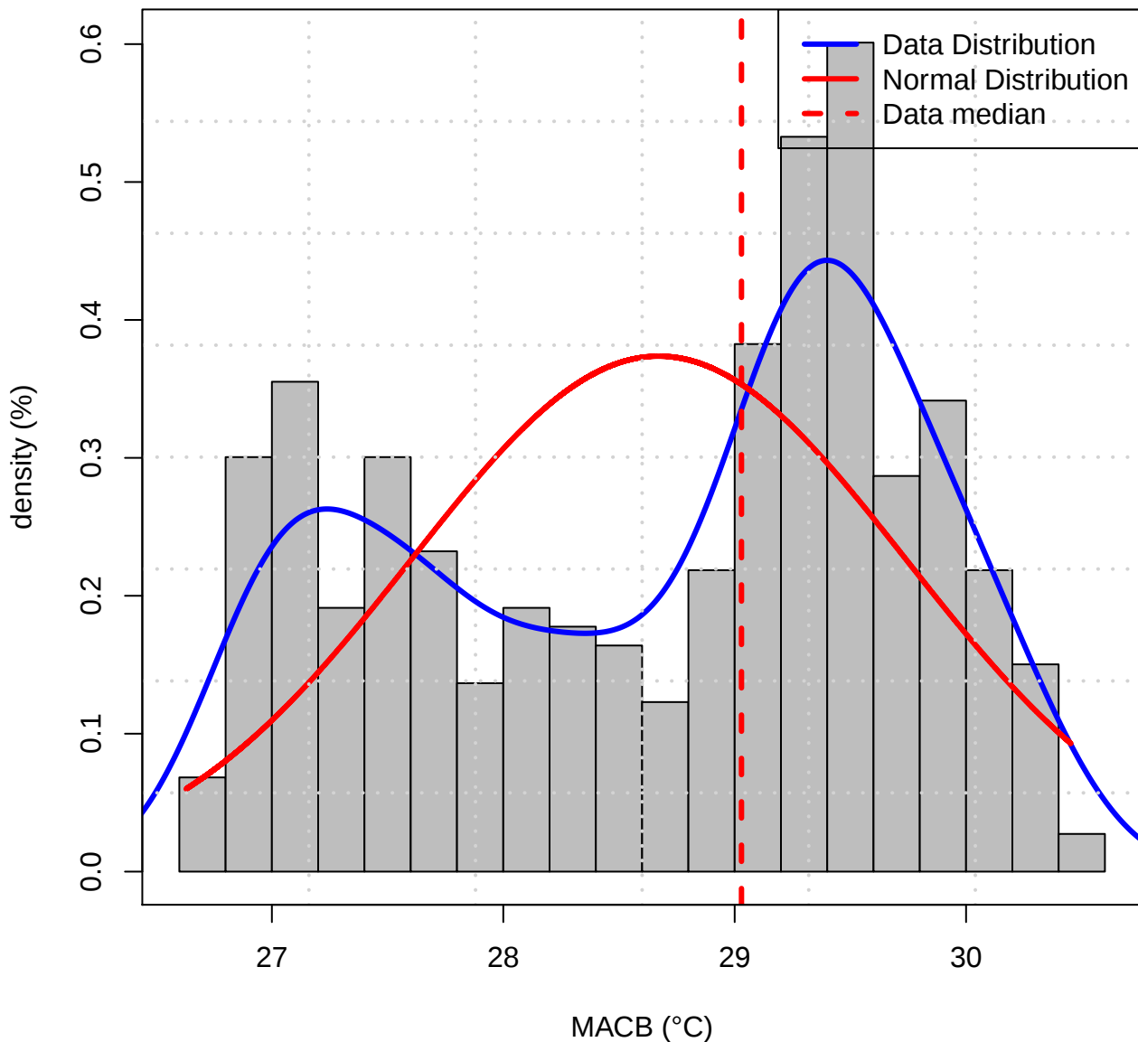
Histogram of Data distribution (TASMAX of MACB)
