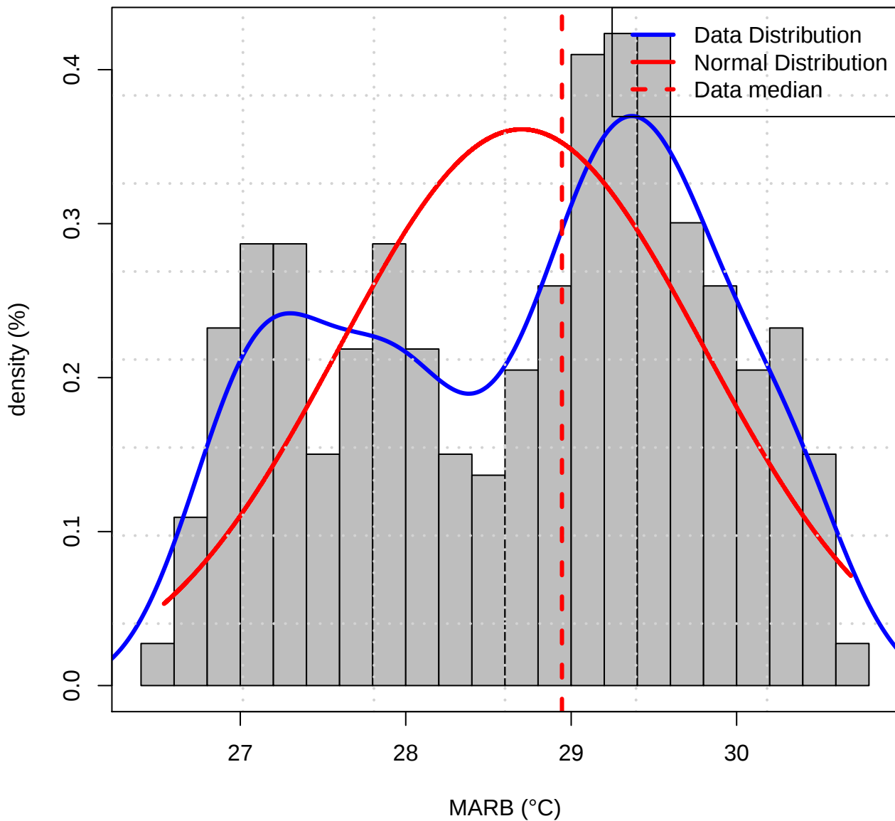
Histogram of Data distribution (TASMAX of MARB)
